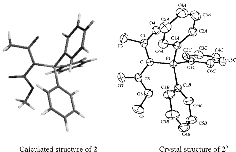
FIGURE 1 The molecular structure of methyl 2-triphenylphosphoranylidene-3-oxobutyrates ( 2 ) showing calculated and crystal geometries. For the crystal structure hydrogen atoms have been omitted for clarity. (Reproduced by permission from the International Union of Crystallography.)
