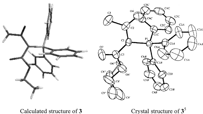
FIGURE 2 The molecular structure of ethyl 2-triphenylphosphoranylidene-3-oxobutyrates ( 3 ) showing calculated and crystal geometry. For the crystal structure hydrogen atoms have been omitted for clarity. (Reproduced by permission from the International Union of Crystallography.)
